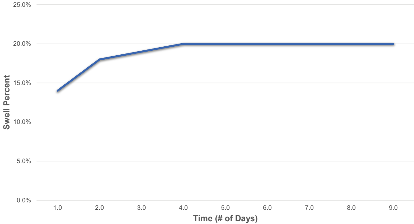
SWELLEX™ Percent Swell (%) in Oil @ 300°F
